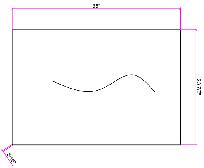
END PANEL 24*35*3/16
